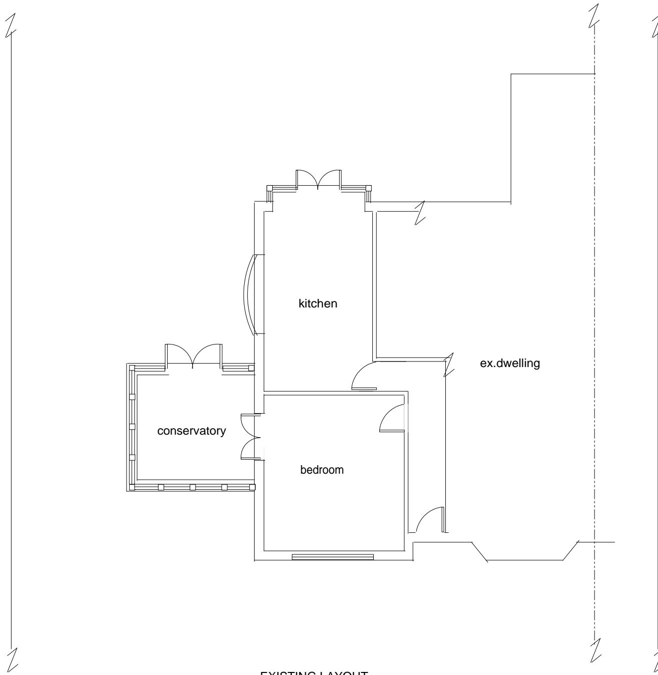
EXISTING LAYOUT
